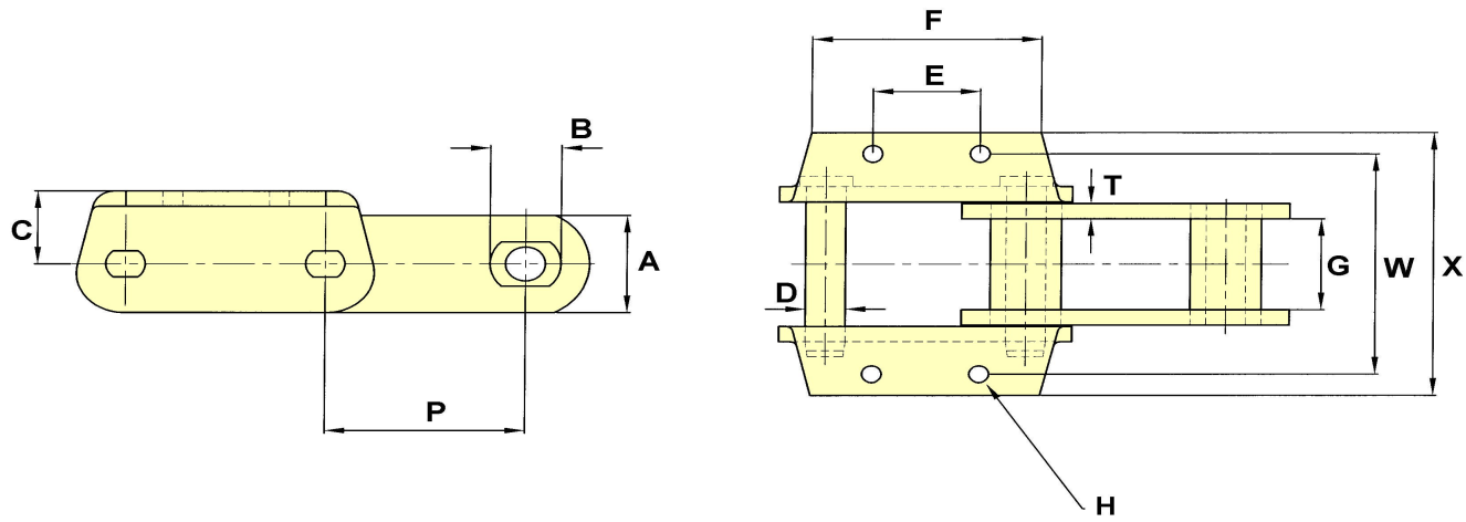
DRAWING NO. 159
