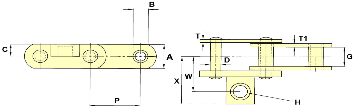
DRAWING NO. 184
