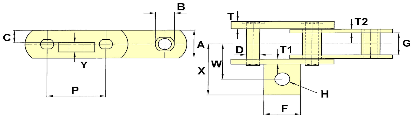
DRAWING NO. 259
