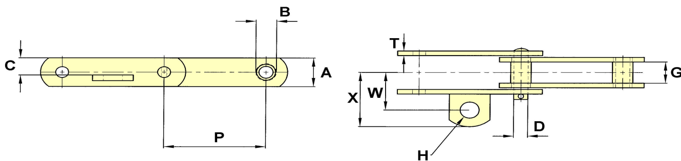
DRAWING NO. 177
