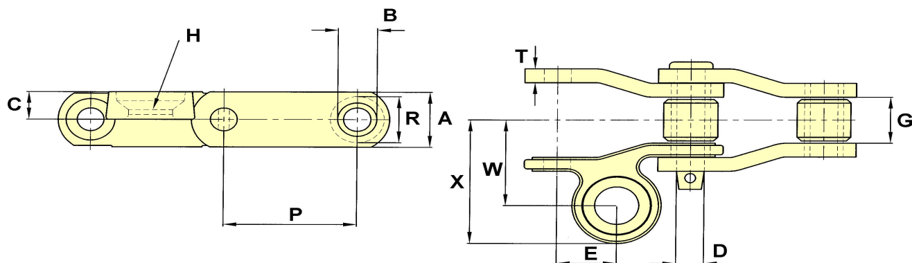
DRAWING NO. 178
