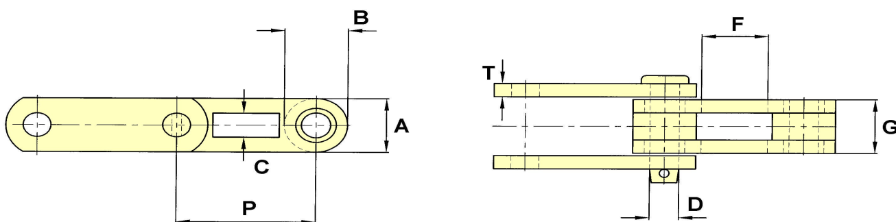
DRAWING NO. 176
