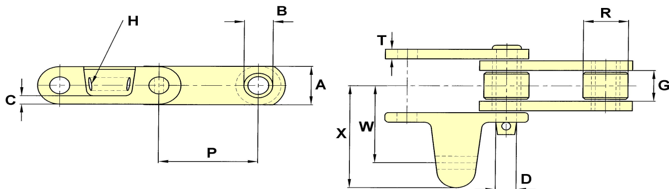
DRAWING NO. 174
